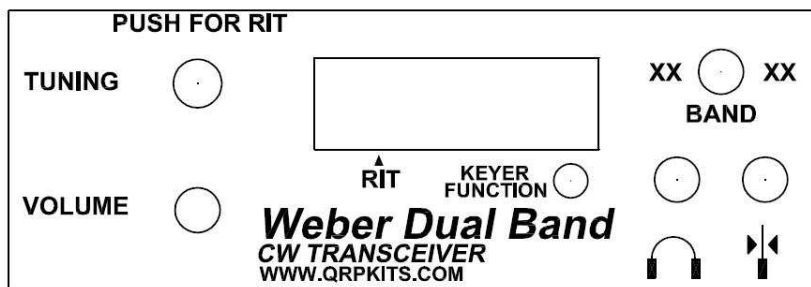
DECAL LAYOUT 1:1
