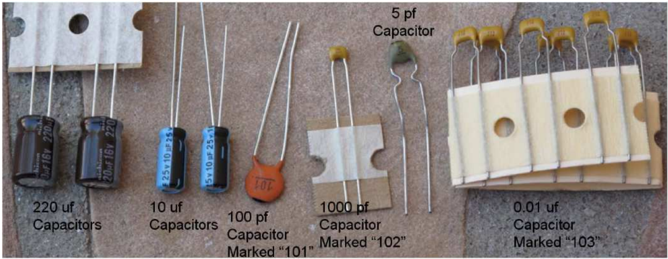
Figure 3. Kit Capacitors
