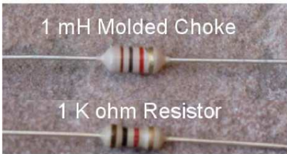
Figure 37. Comparison between a 1K resistor and a 1 mH molded choke
