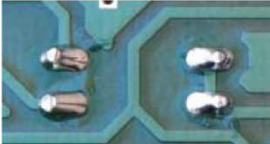
Figure 15. View of trimmed leads after soldering
