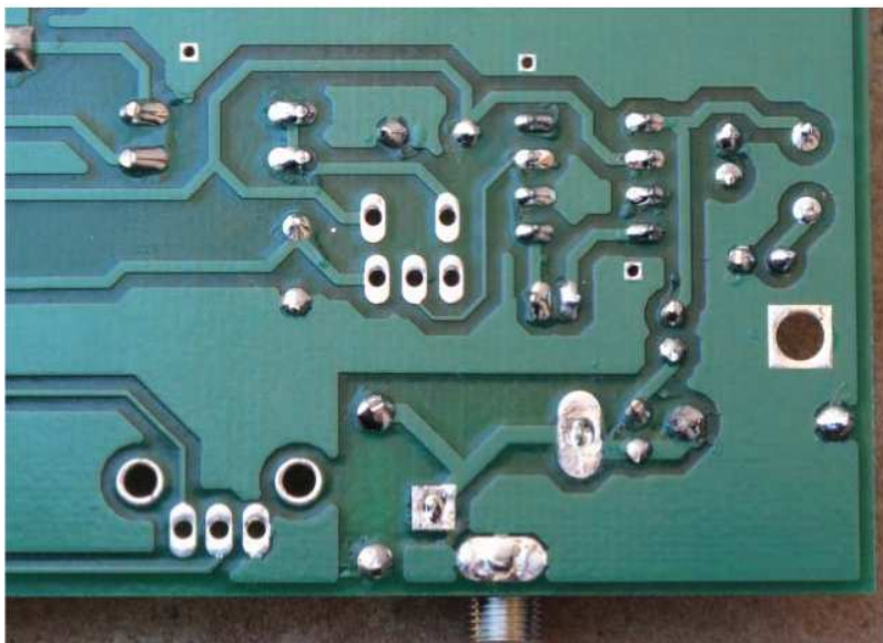
Figure 25. Bottom side view of Audio amplifier section
