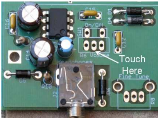
Figure 29. Where to touch for the “hum test”
