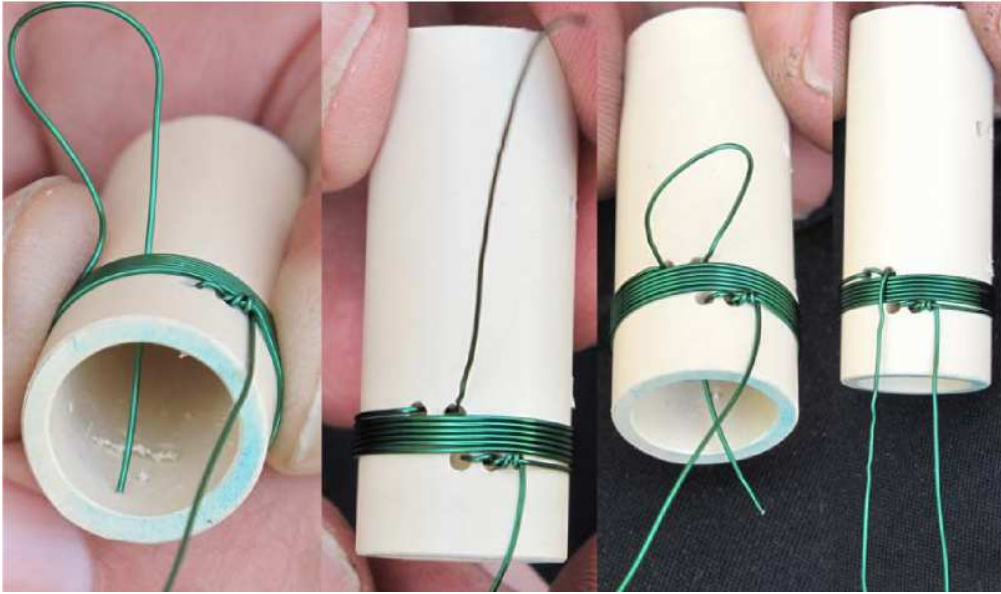
Figure 52. Tying off far end of first winding of L1
