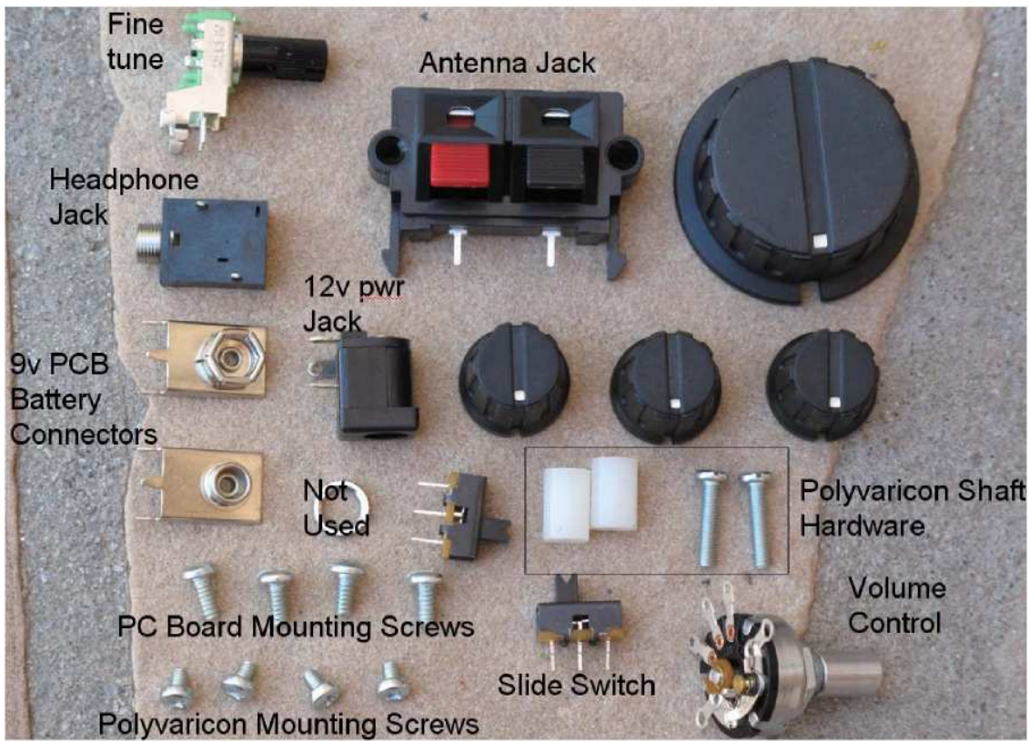
Figure 1. Kit hardware
