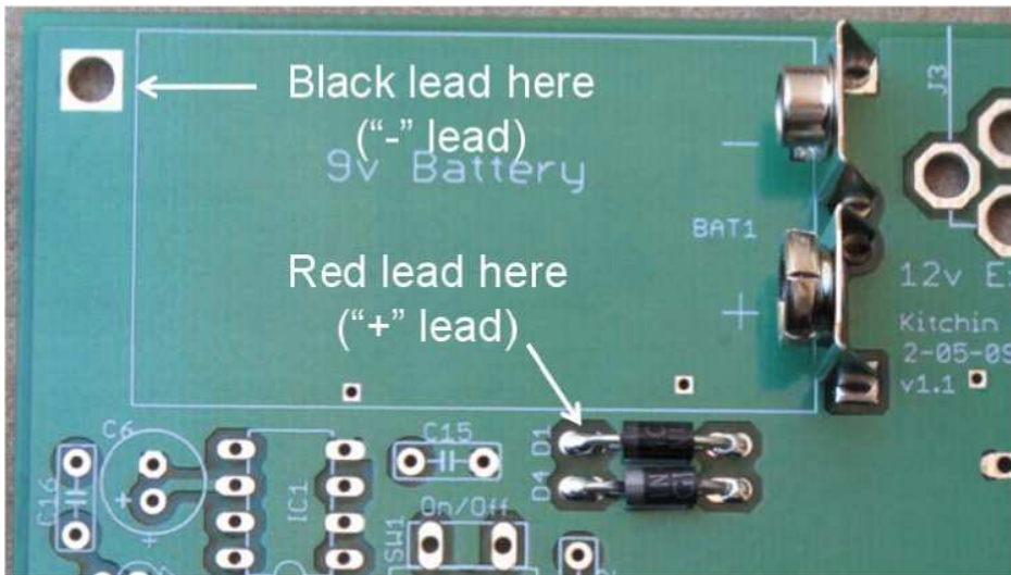
Figure 17. Test points for voltage measurement
