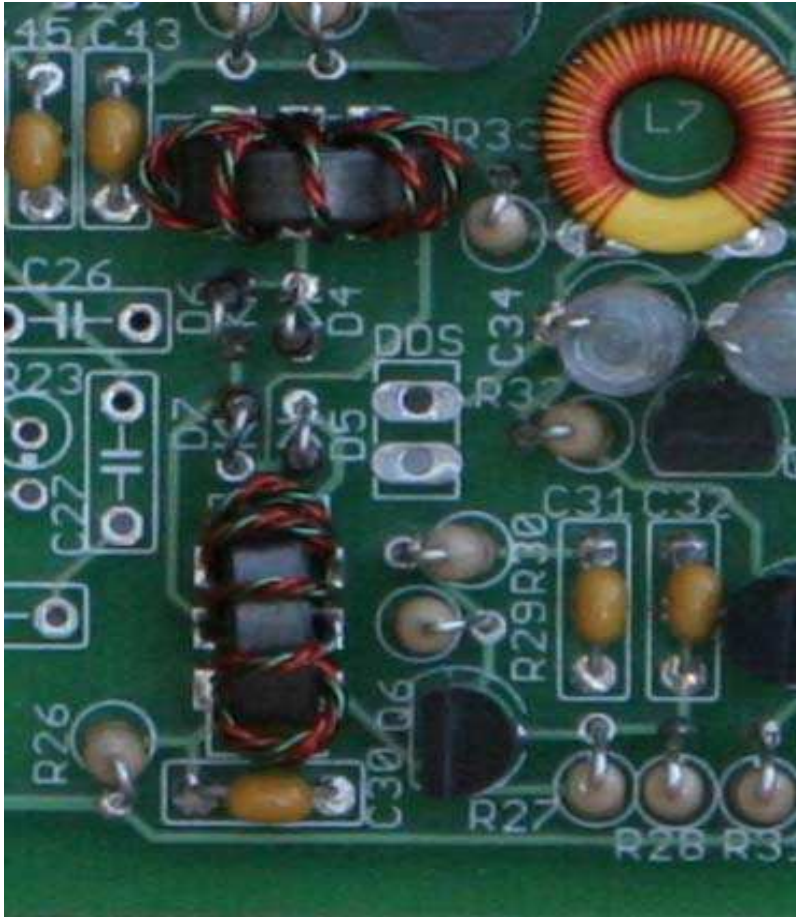
Illustration 10: First Mixer (VFO Mixer), (N7VE Photo)
