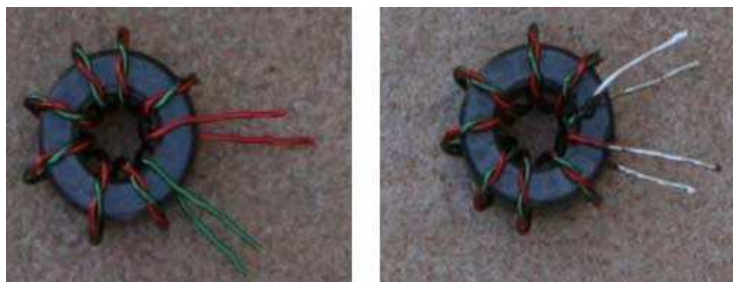
Illustration 19: T-3 Winding Detail (N7VE Photo)
